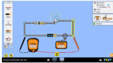
Figure 3. Experimental Circuit Design 2
