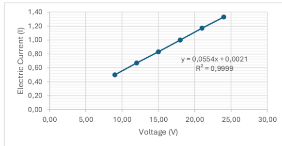
Figure 4. Graph of Voltage Relationship to Electric Current
