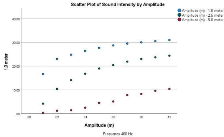
Figure 5. Graph of the Relationship Between Sound Intensity and Amplitude at a Frequency of 400 Hz
