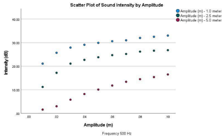
Figure 6. Graph of the Relationship Between Sound Intensity and Amplitude at a Frequency of 500 Hz
