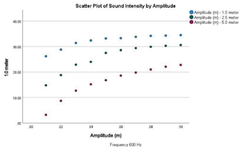
Figure 7. Graph of the Relationship Between Sound Intensity and Amplitude at a Frequency of 600 Hz
