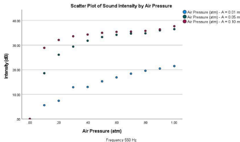
Figure 9. Graph of the Relationship Between Sound Intensity and Air Pressure
