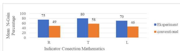
Figure 1: Average percentage <g> of each indicator of connection mathematics.
