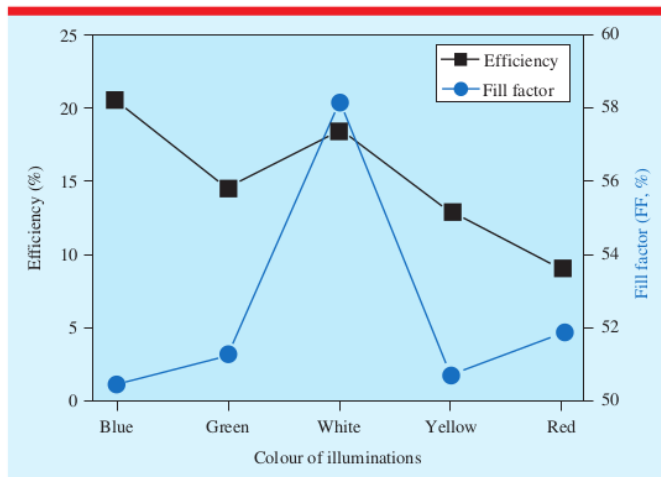
Figure 5. Solar cell properties for several illumination colors.
