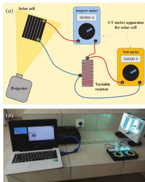
Figure 2. (a) The I-V measurement schematic, and (b) the I-V measurement prototype for solar cells tested with the LCD projector as the illumination source.
