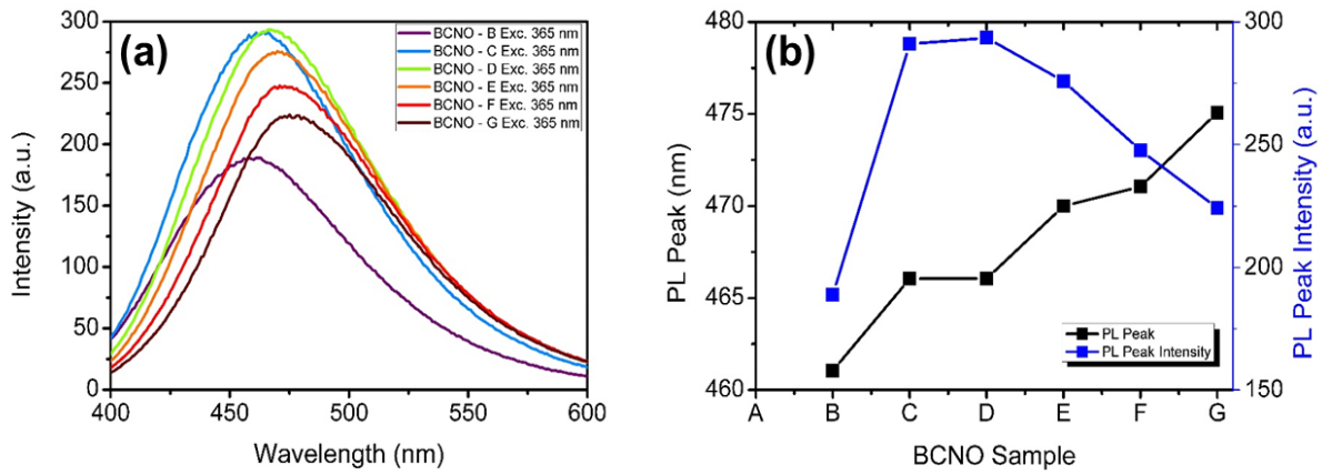
Figure 3. Effect of carbon concentration on the Photoluminescence properties of BCNO nanoparticle: (a) PL Spectra and (b) PL Properties.
