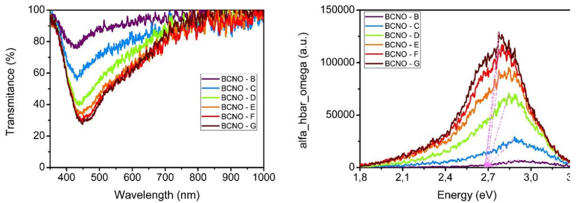
Figure 5. Transmittance spectra and tauc plot analysis of BCNO phosphor material (Sample D).
