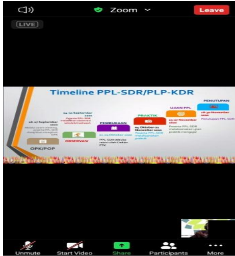
Gambar 1.1 OPK PPL-SDR
