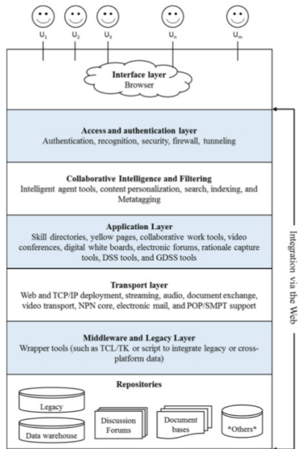
Fig. 7. Knowledge Management System Architecture (Tiwana, 1999)
