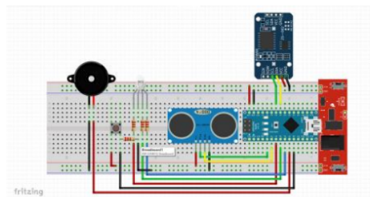
Figure 2. Assembly of The Trash Bin Monitor
