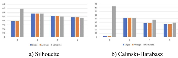
FIG 5. SILHOUETTE AND CALINSKI-HARABASZ FOR COSINE
