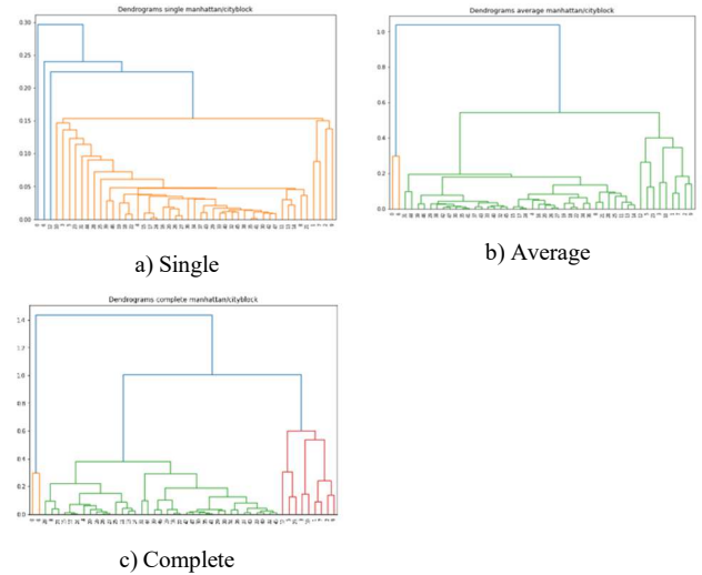
FIG 6. DENDROGRAM OF MANHATTAN/CITYBLOCK
