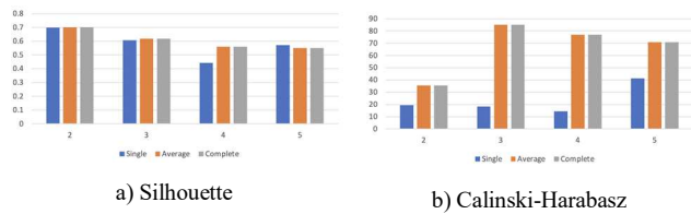
FIG 7. SILHOUETTE AND CALINSKI-HARABASZ FOR MANHATTAN
