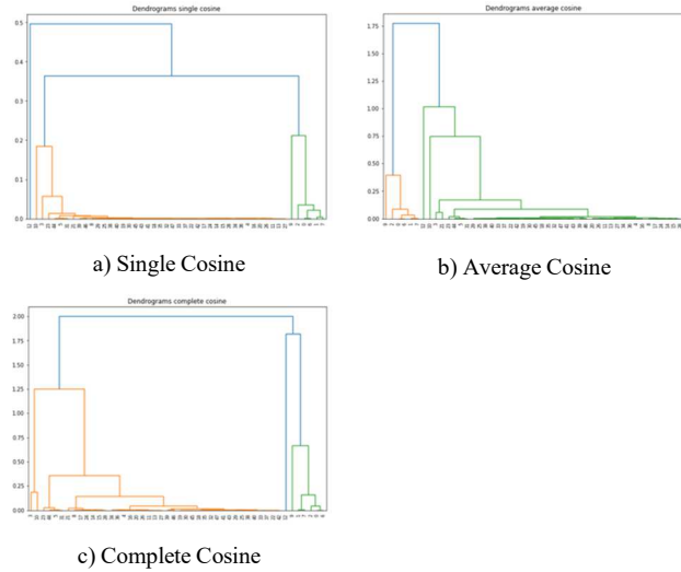
FIG 4. DENDROGRAM OF COSINE
