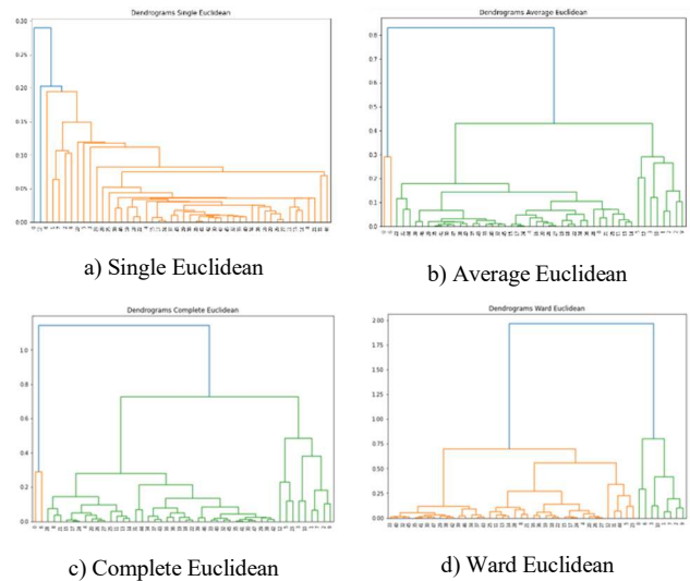
FIG 2. DENDROGRAM OF EUCLIDEAN
