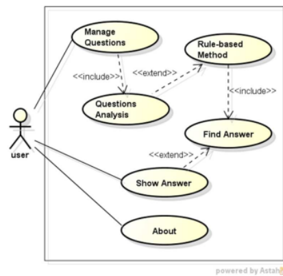
Figure 3. Use case Diagram
