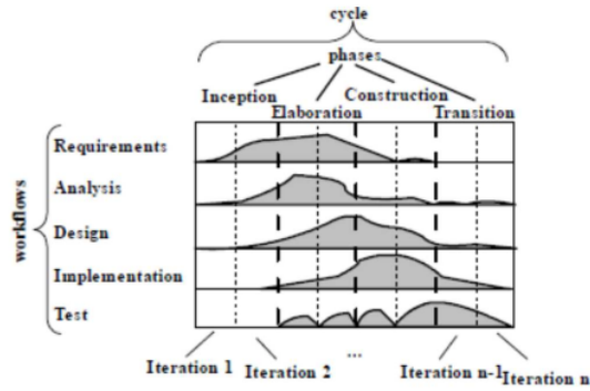
Figure 2. RUP modelling process [20]
