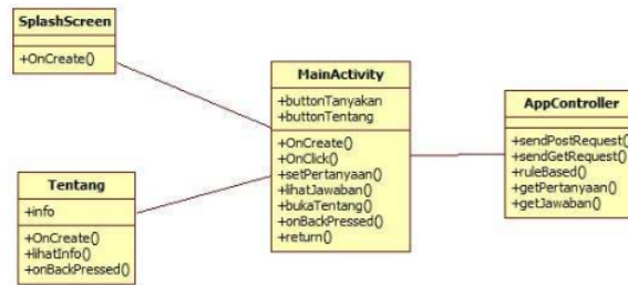
Figure 1. Class Diagram
