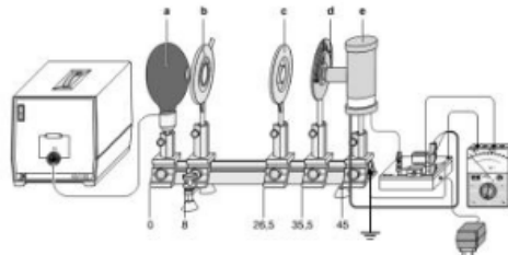
Gambar 1. Planck Constant Measuring
