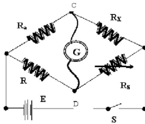
Gambar 3. Prinsip Rangkaian Jembatan Wheatstone
