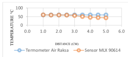
Fig. 4. Graph of temperature measurement test results between sensor and mercury thermometer
