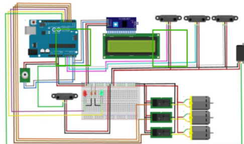
Fig. 1. Prototype Design Scheme
