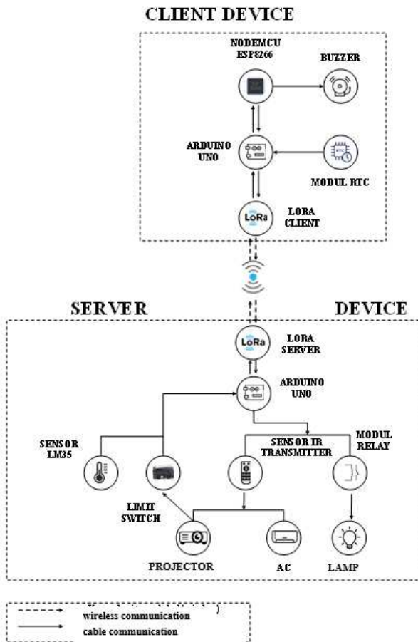
Fig. 5. Block communication device
