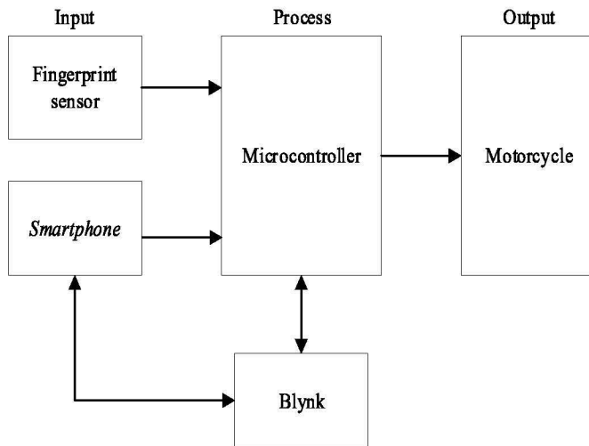
Fig. 2. Block diagram control system design
