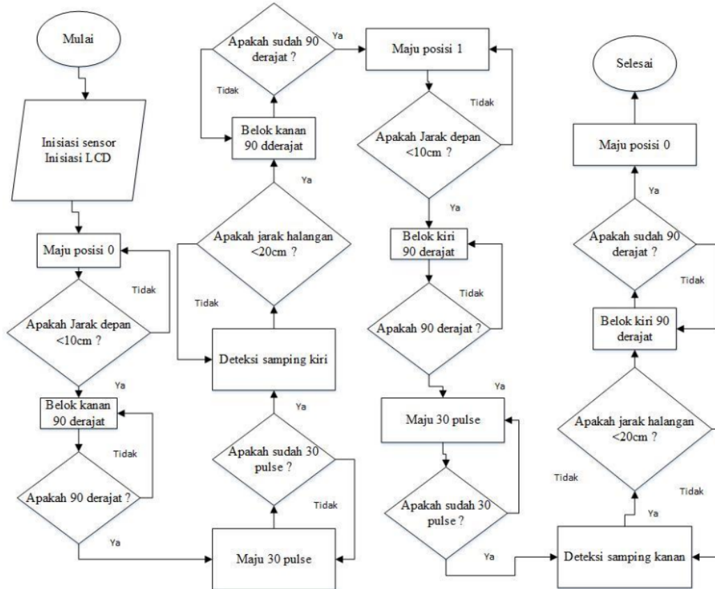
Gambar 6. Alur kerja program
