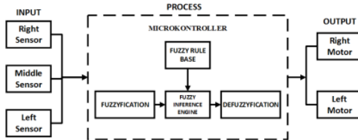
4 Fig. 1. The block diagram of this control system.
