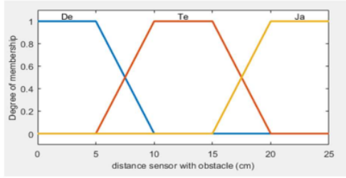
Fig. 4. Membership function of left sensor.
