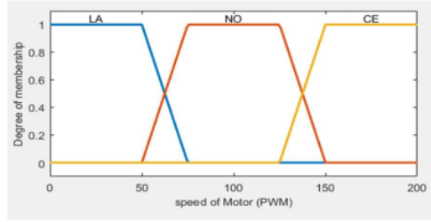
Fig. 7. MF output of right motor speed.
