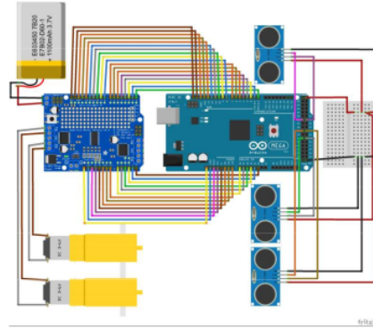
Fig. 2. Circuit System.
