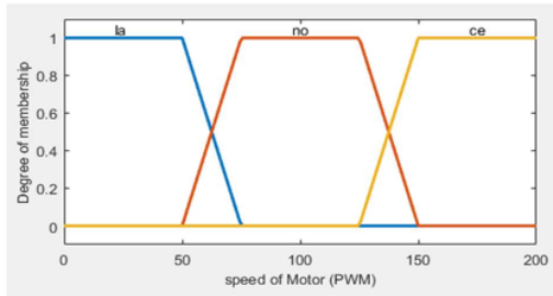
Fig. 6. MF output of left motor speed.
