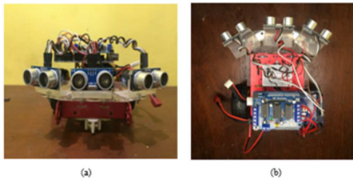
Fig. 8. Robot (a) front view; (b) top view.
