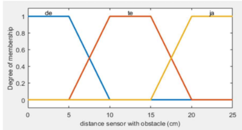
Fig. 5. Membership Function of middle sensor.
