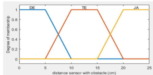
Fig. 3. Membership function of right sensor.
