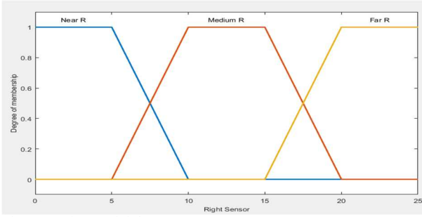
Fig. 4. MF input of right sensor.
