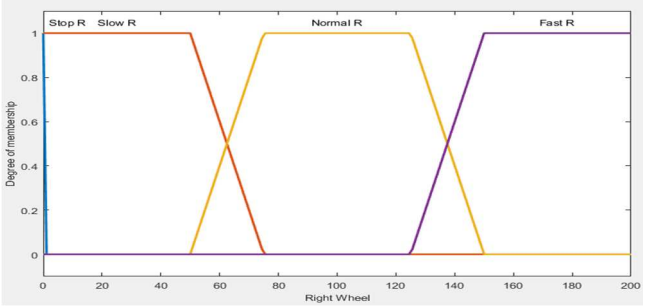
Fig. 8. MF output of right motor speed
