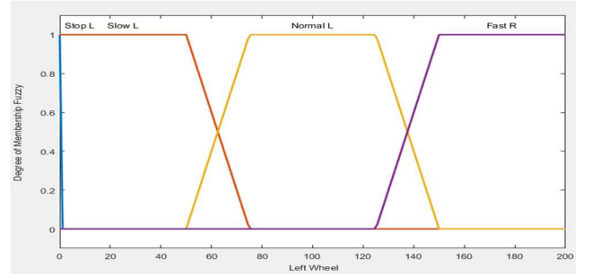
Fig. 7. MF output of left motor speed.
