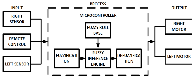
Fig. 1. The block diagram of this control system.
