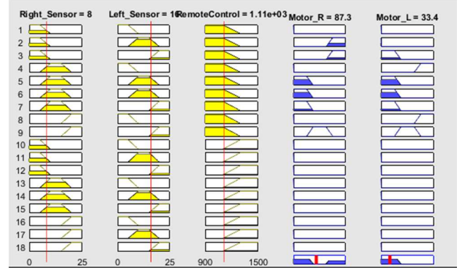
Fig. 9. MF Result of Fuzzy design in MatLab
