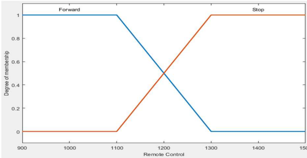
Fig. 6. MF input of remote control
