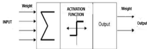
Fig. 2. ANN's structure.
