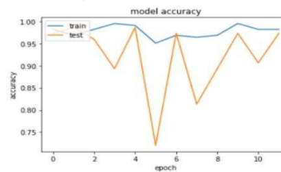
Fig. 9. Graphics of accuracy model
