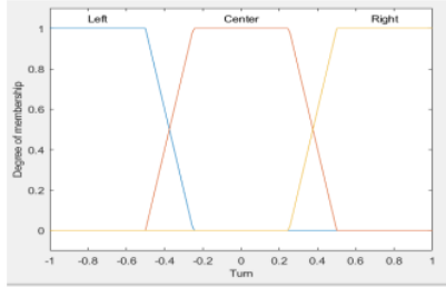
Fig. 4. Membership function of Turn.
