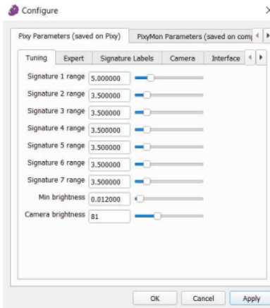
Fig. 8. PixyMon tuning.
