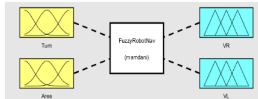
Fig. 3. Fuzzy logic design.
