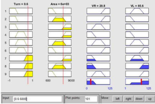
Fig. 9. Software simulation.
