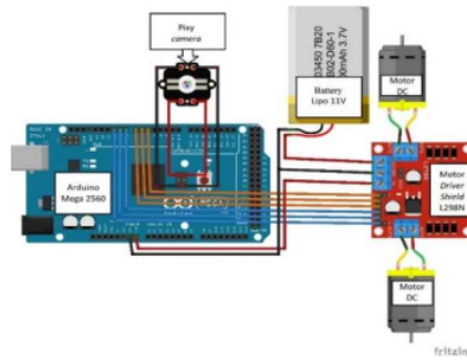
Fig. 2. Schematic system.
