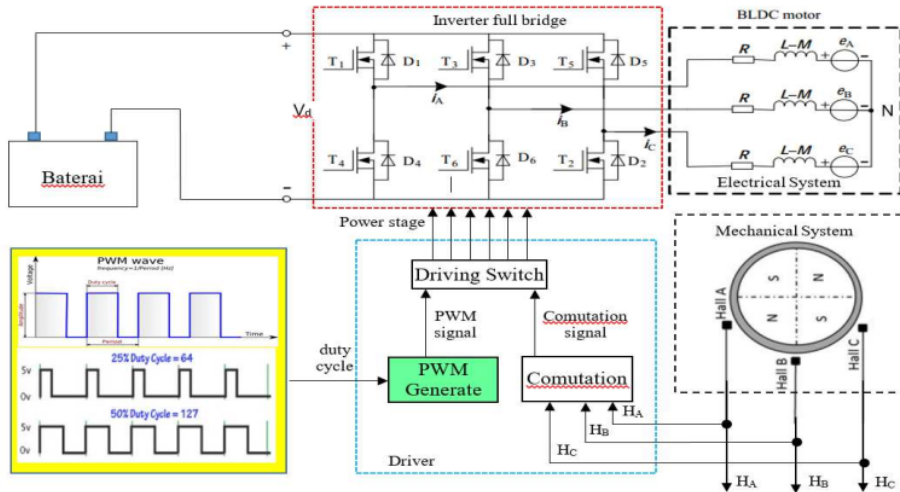
Fig. 4. BLDC motor driver [11].
