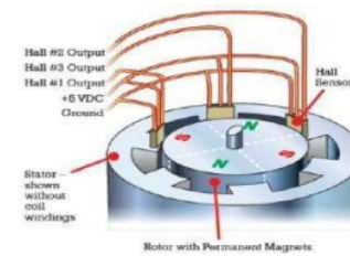
Fig. 2. Sensor hall and its position.
