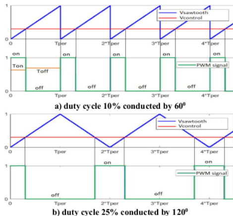
Fig. 5. PWM signal generator [10].
