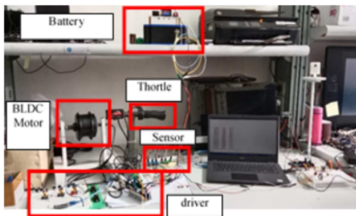
Fig. 7. Testbed.
