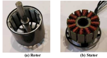
Fig. 1. Motor main part.
