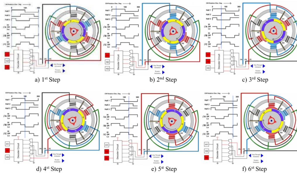
Fig. 3. Procedure BLDC motor [9].
