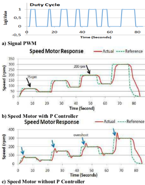
Fig. 9. Duty cycle and speed motor response.
