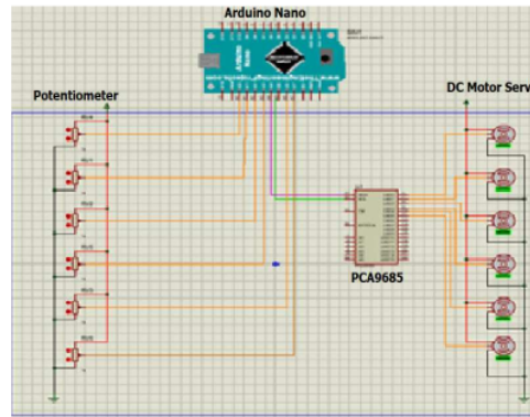
Fig. 6. Diagram block drive module.
