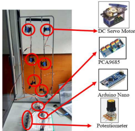
Fig. 5. Experimental setup.
