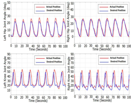
Fig. 8. Kinematics tracking performance.
