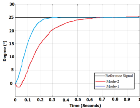
Fig. 7. PID controller response with ZN method.
