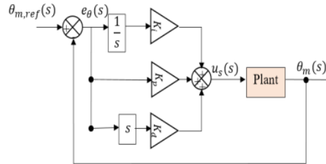
Fig. 4. PID controller design.
