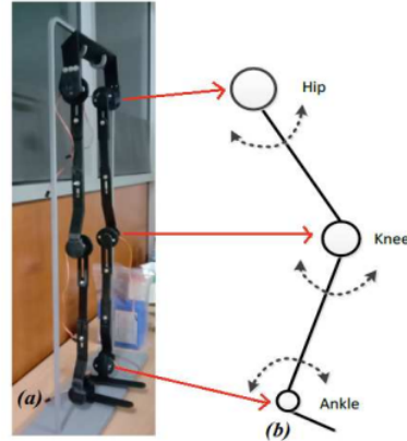
Fig.1. 3D Lower-limb Exoskeleton
